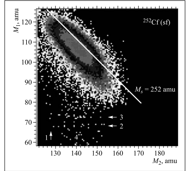
Fig. 3. Mass–mass distribution for the fragments from ^{252}\text{Cf} (sf) around the «Ni bump»
