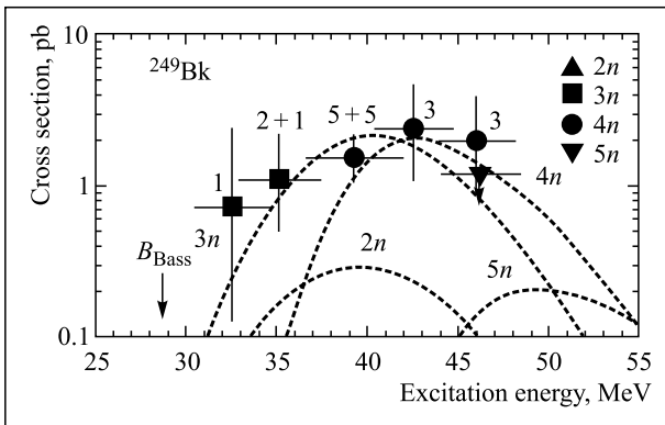
Fig. 2. Production cross sections of ^{294}_{117} and ^{293}_{117} vs. excitation energy of the compound nucleus. Figure specifies the number of nuclei synthesized in the present experiment and in 2010
