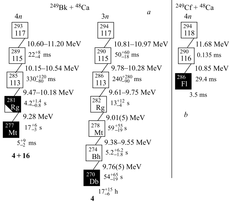
Fig. 1. (a) Radioactive properties of ^{293,294}_{117} and their daughter nuclei. Energies of \alpha particles and half-lives are given in the figure. The spontaneously fissioning isotopes are shown as black squares. (b) Decay chain of ^{294}_{118} (with \alpha -particle energies and decay times)
